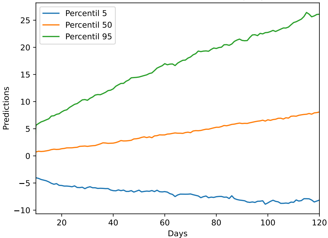
Predictions with 95% Confidence. Company: ACWI
