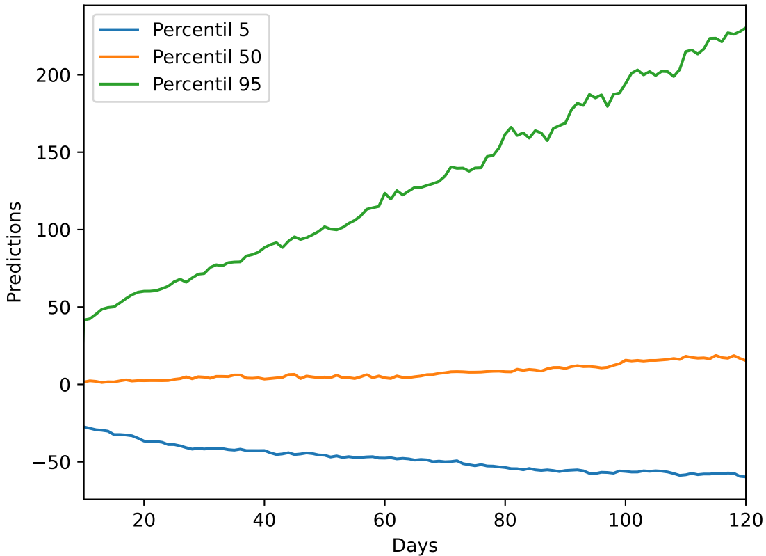
Predictions with 95% Confidence. Company: SOXL
