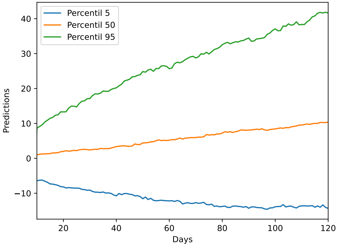
Predictions with 95% Confidence. Company: XLK
