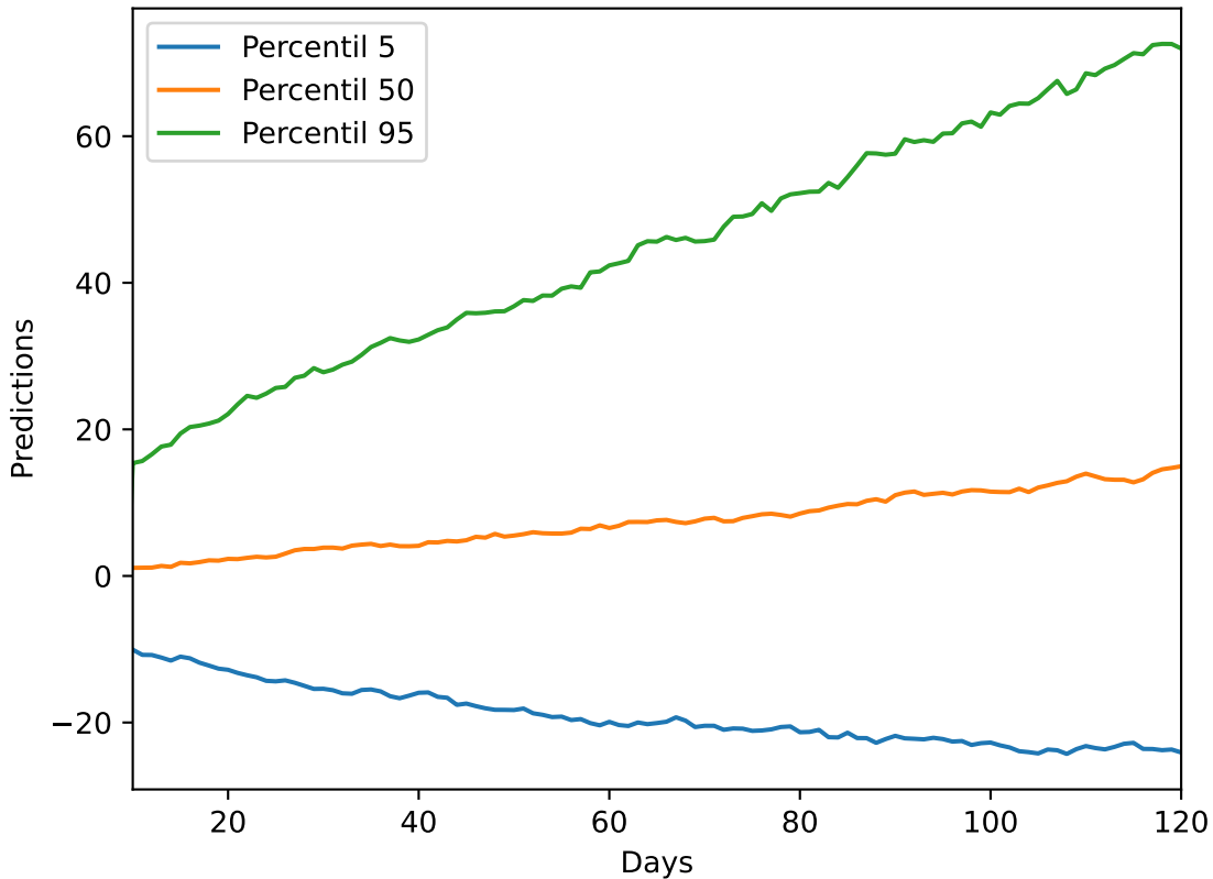
Predictions with 95% Confidence. Company: SIL
