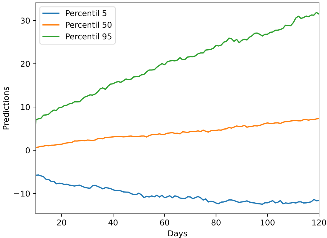
Predictions with 95% Confidence. Company: IVW
