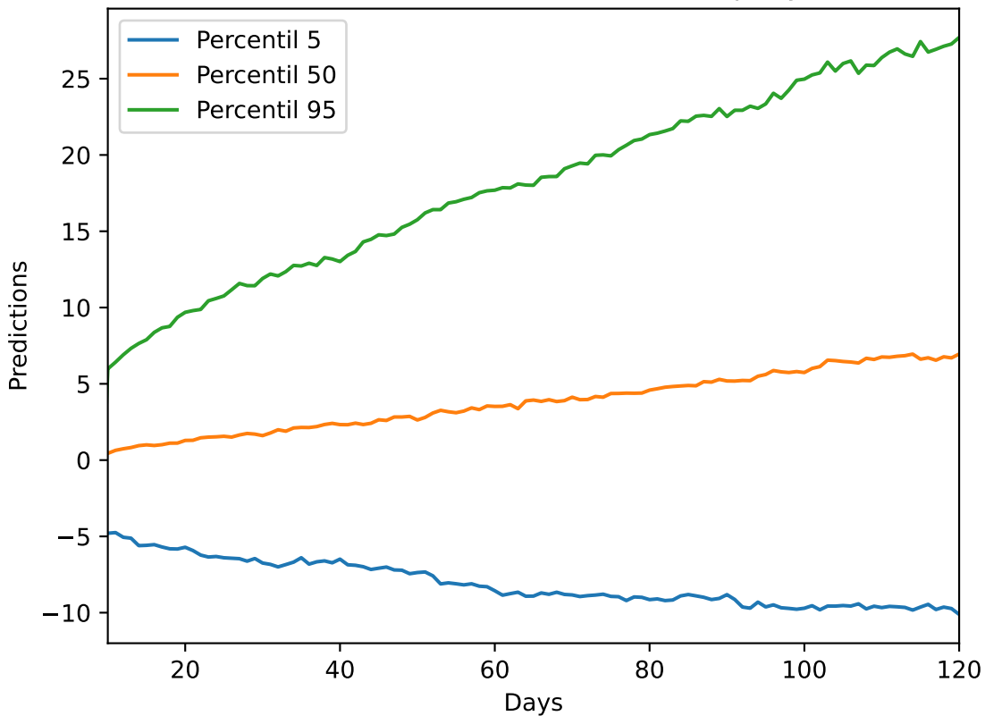
Predictions with 95% Confidence. Company: EWC
