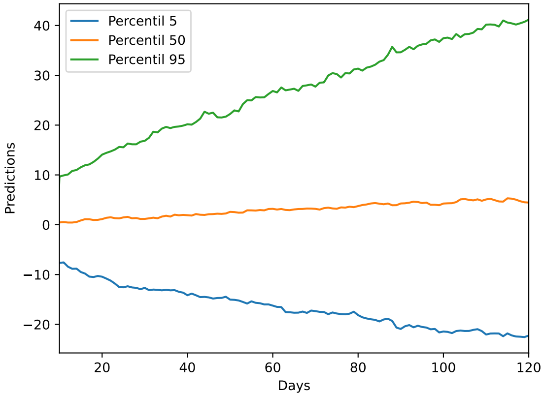
Predictions with 95% Confidence. Company: EPOL
