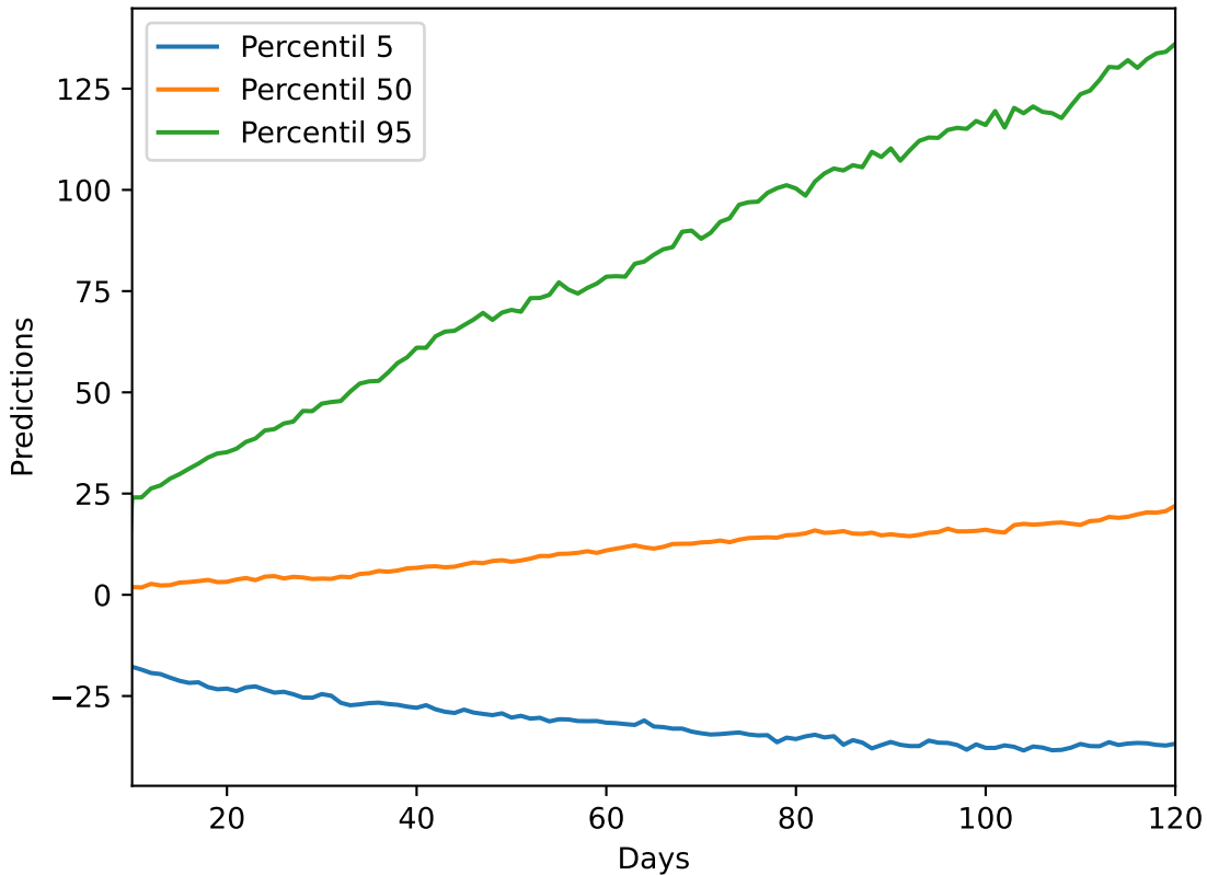
Predictions with 95% Confidence. Company: TQQQ
