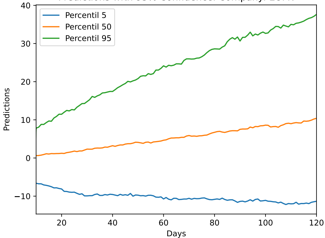
Predictions with 95% Confidence. Company: EUFN
