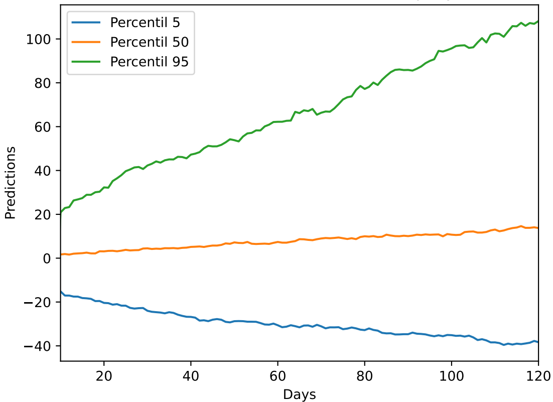
Predictions with 95% Confidence. Company: FAS
