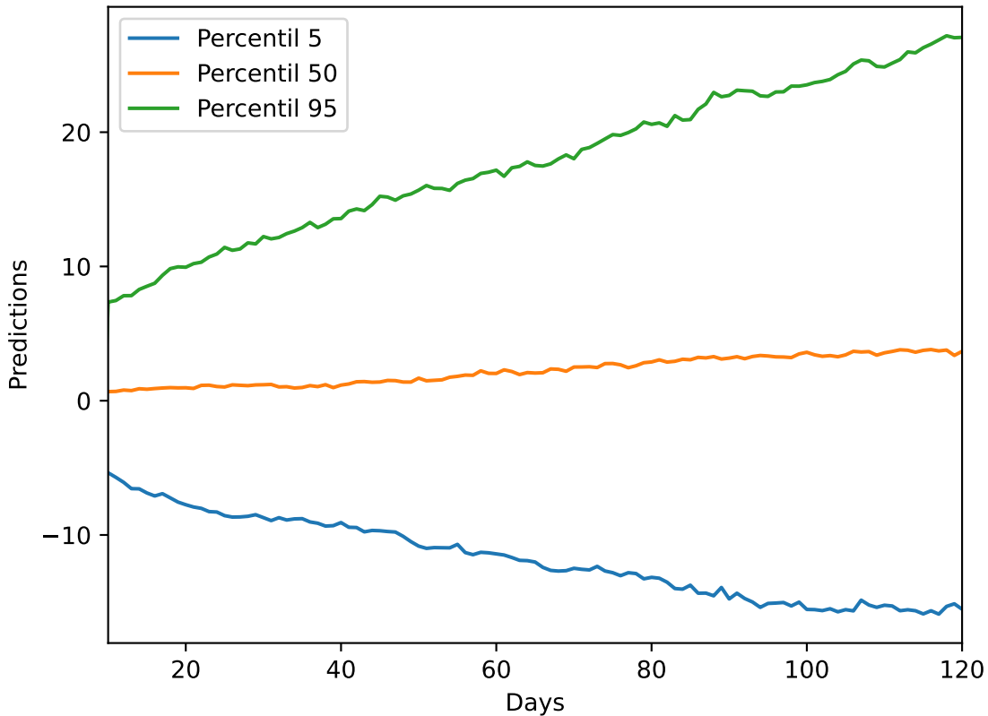
Predictions with 95% Confidence. Company: EWG
